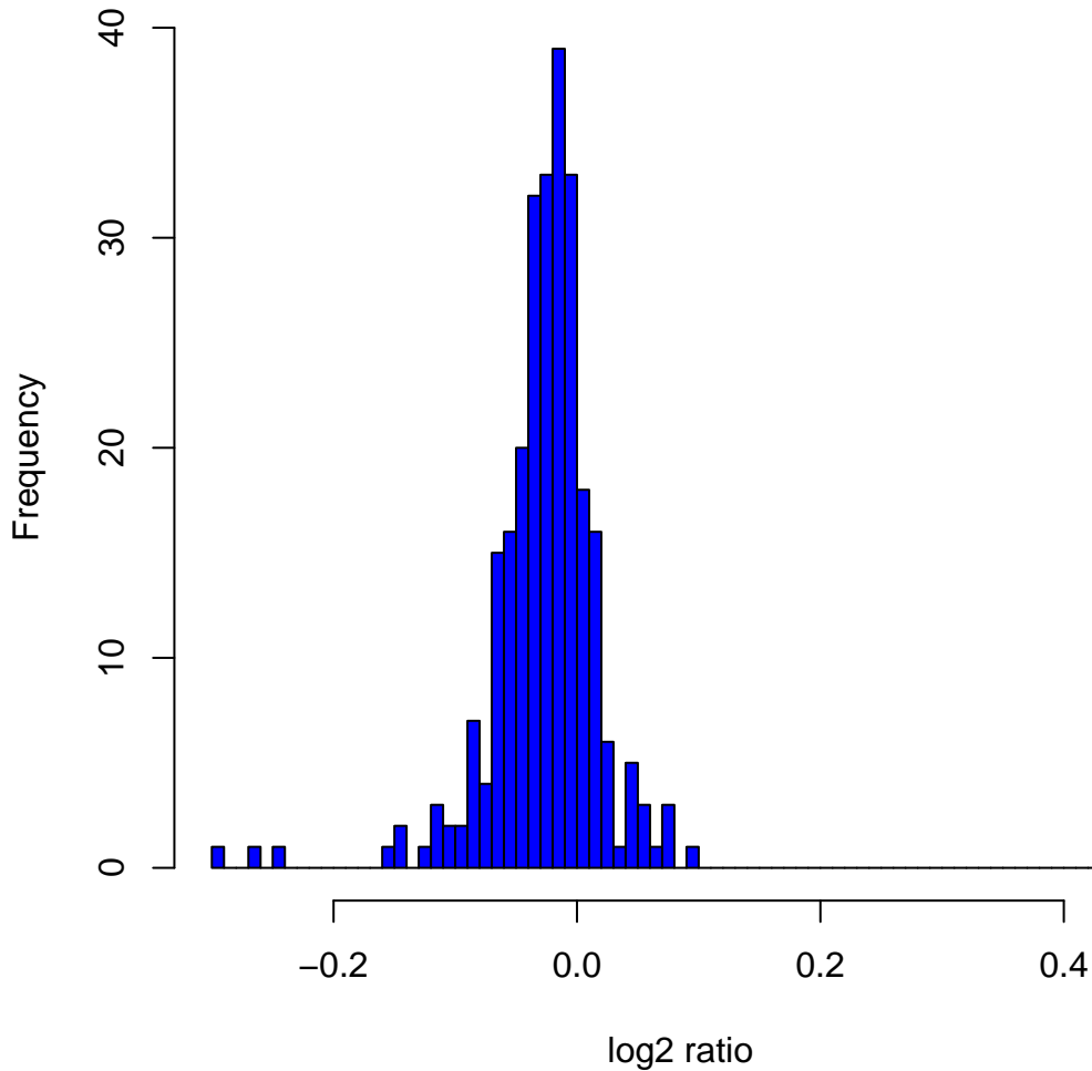
Histogram of \log_2 ratios in 270 HapMap samples at clone Chr12tp-16A9
