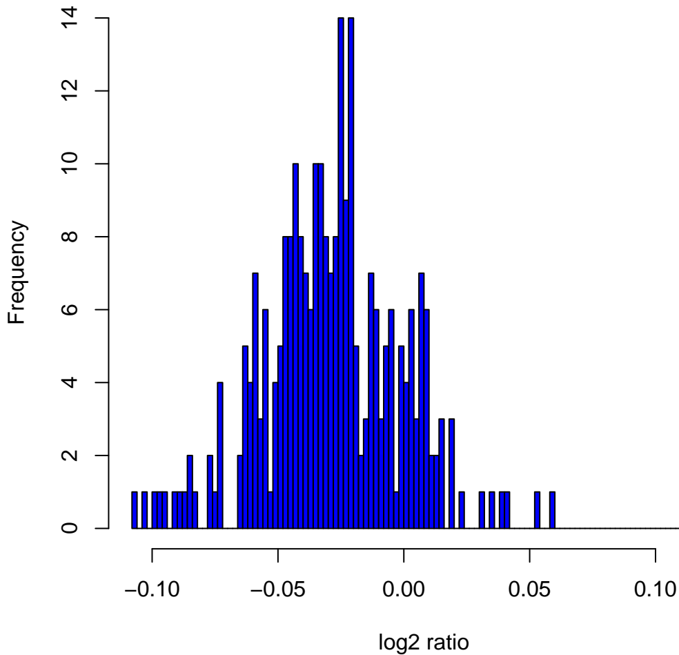
Histogram of log2ratios in 270 HapMap samples at clone Chr12tp-16B10
