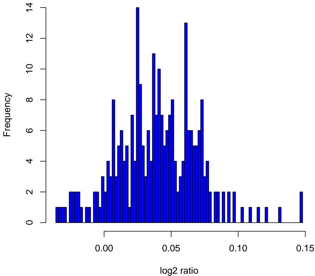
Histogram of log2ratios in 270 HapMap samples at clone Chr12tp-16B2
