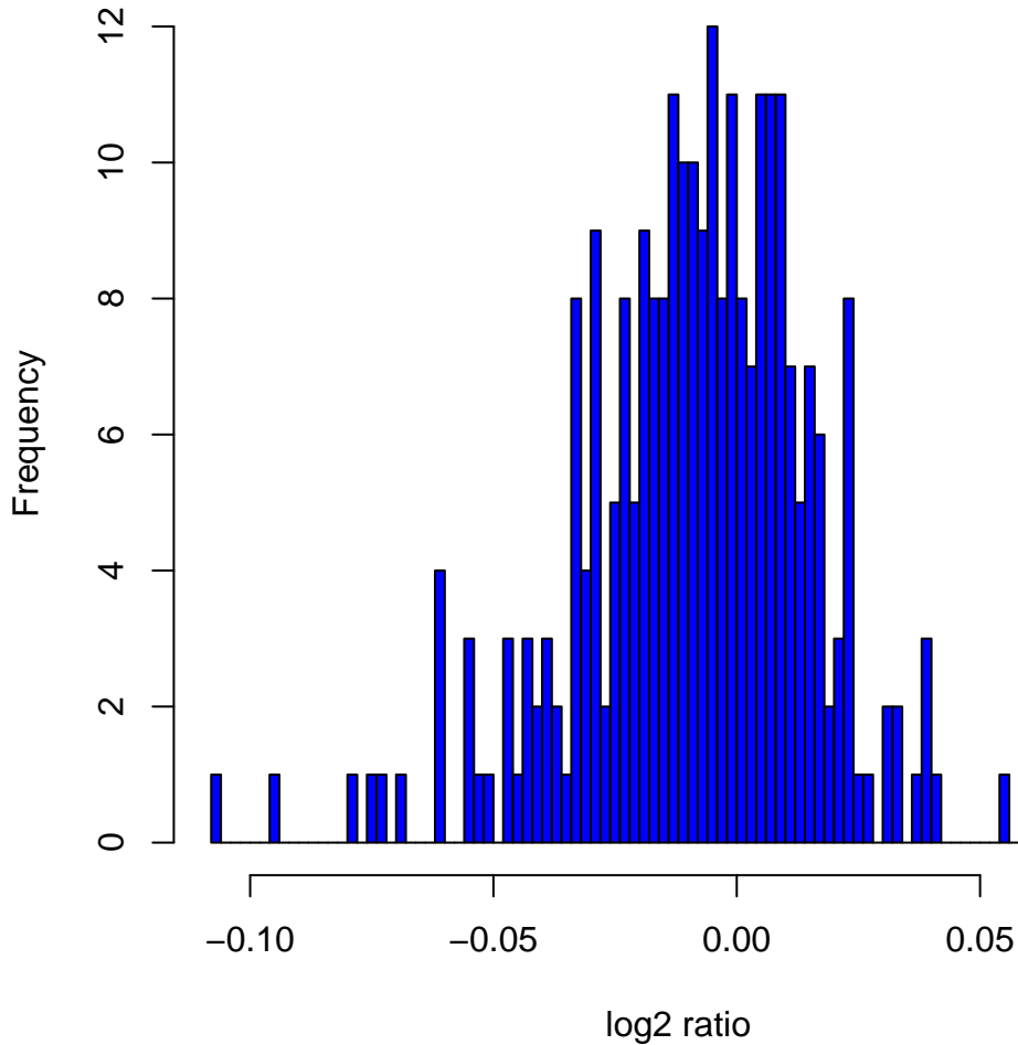
Histogram of log2ratios in 270 HapMap samples at clone Chr12tp-16E2
