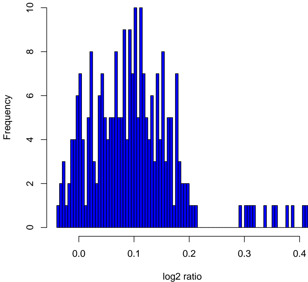
Histogram of log2ratios in 270 HapMap samples at clone Chr12tp-16E7
