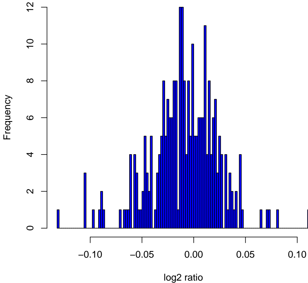
Histogram of log2ratios in 270 HapMap samples at clone Chr12tp-16F5
