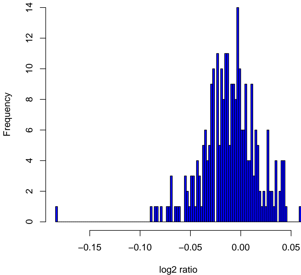
Histogram of log2ratios in 270 HapMap samples at clone Chr12tp-16G11
