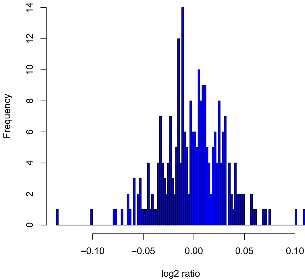
Histogram of log 2 ratios in 270 HapMap samples at clone Chr12tp-17A12
