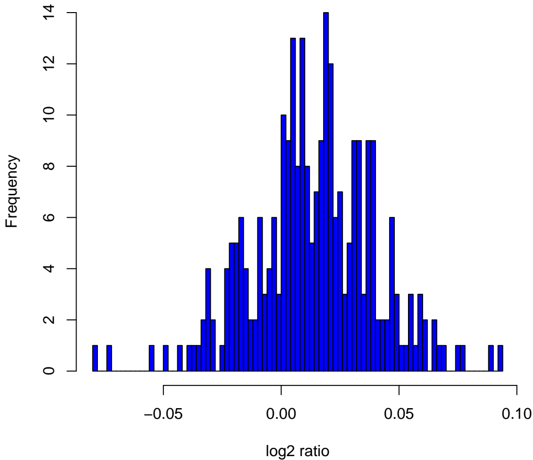
Histogram of log2ratios in 270 HapMap samples at clone Chr12tp-17A7
