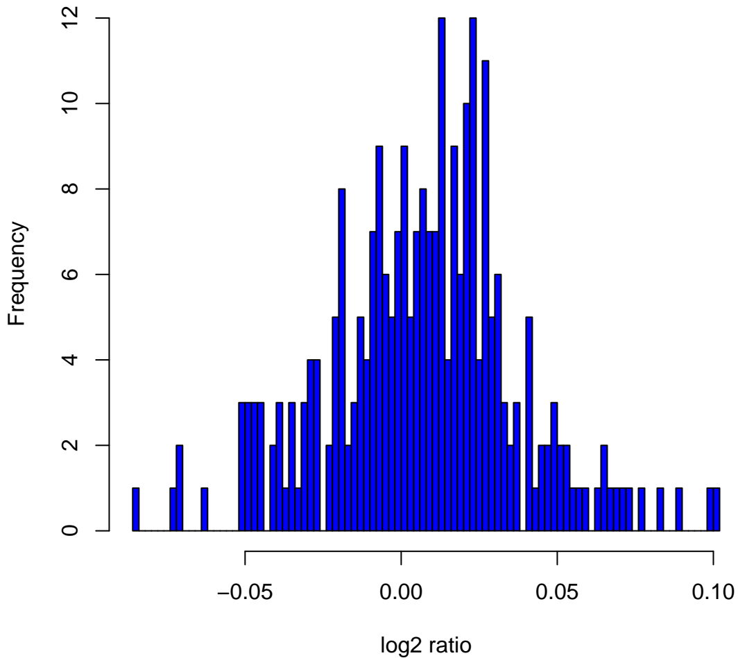
Histogram of log2ratios in 270 HapMap samples at clone Chr12tp-17B4
