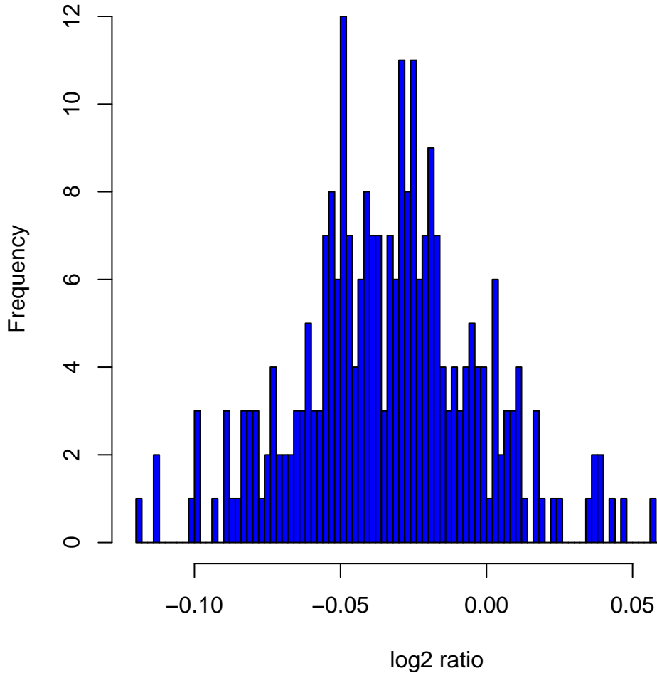
Histogram of log2ratios in 270 HapMap samples at clone Chr12tp-17C4
