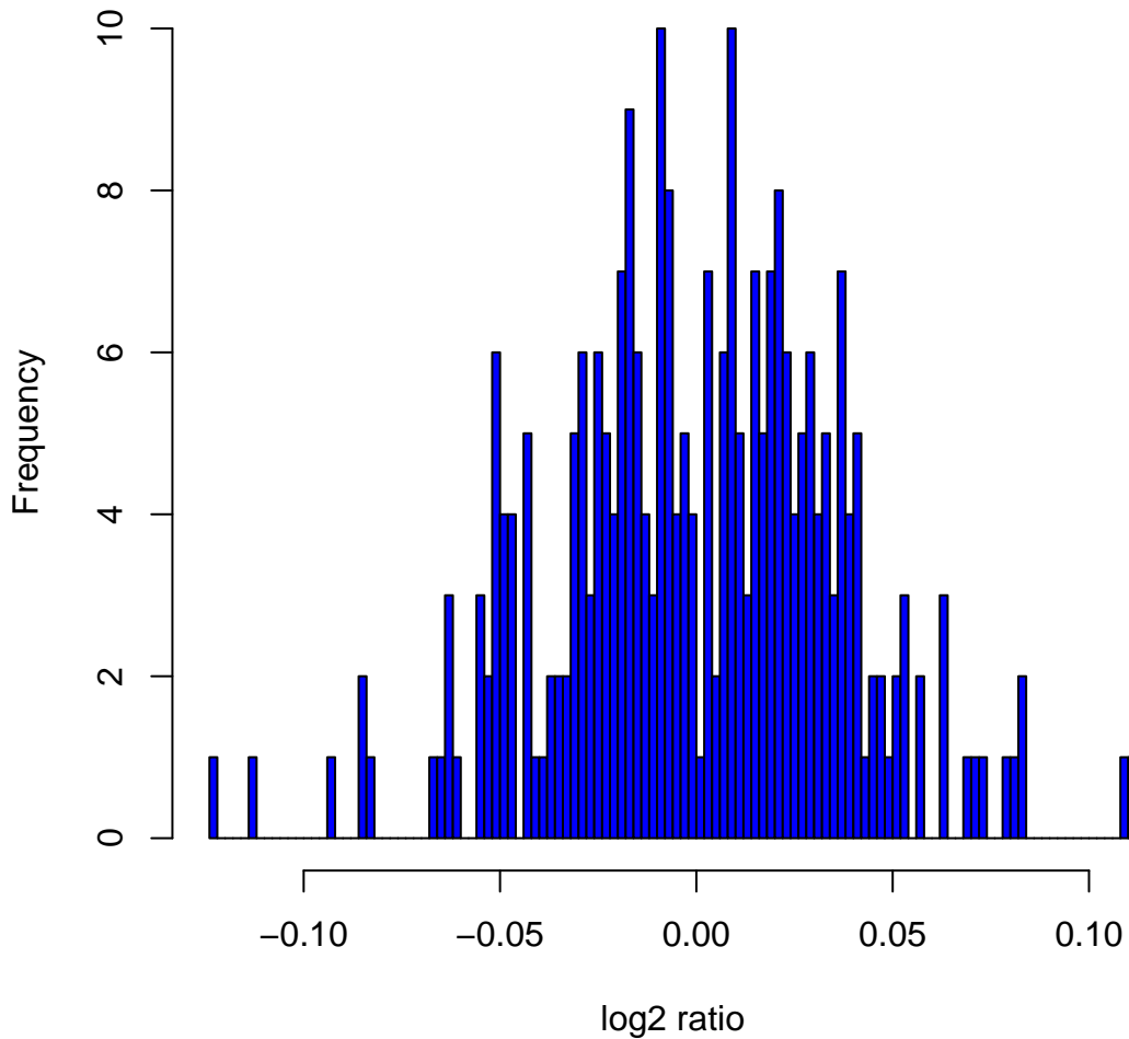
Histogram of log2ratios in 270 HapMap samples at clone Chr12tp-17D4
