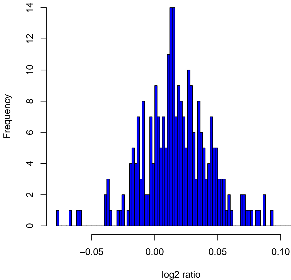
Histogram of log2ratios in 270 HapMap samples at clone Chr12tp-17E7
