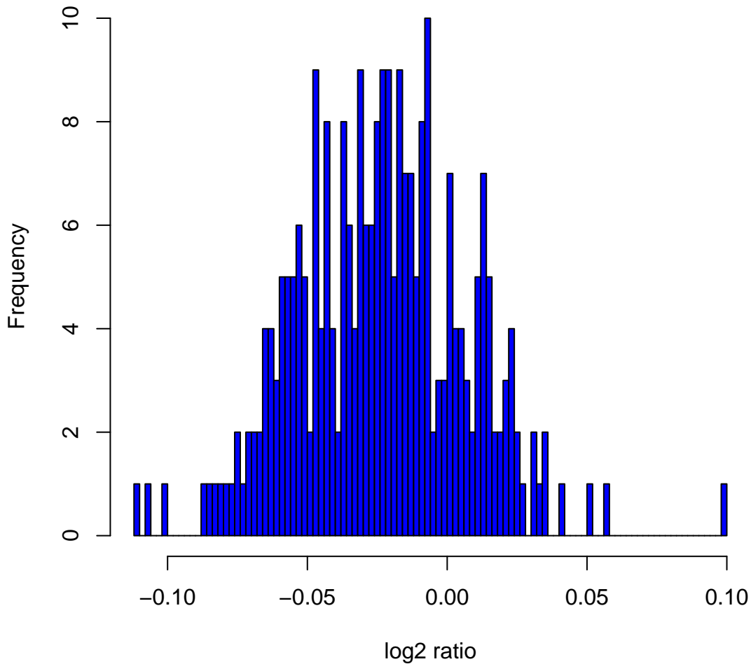
Histogram of \log_2 ratios in 270 HapMap samples at clone Chr12tp-17G5
