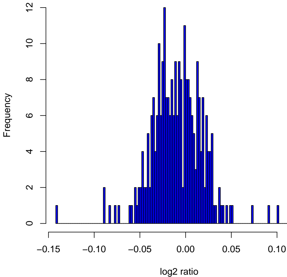
Histogram of log2ratios in 270 HapMap samples at clone Chr12tp-18A4
