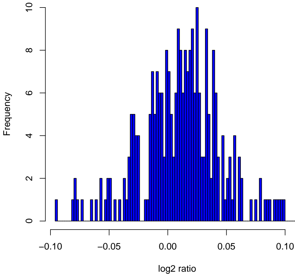
Histogram of log2ratios in 270 HapMap samples at clone Chr12tp-18B2
