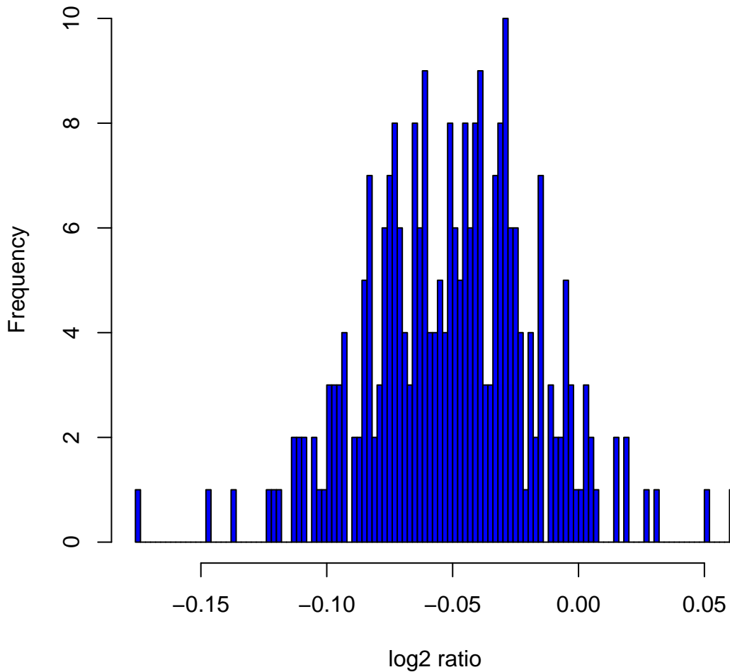
Histogram of \log_2 ratios in 270 HapMap samples at clone Chr12tp-18G3
