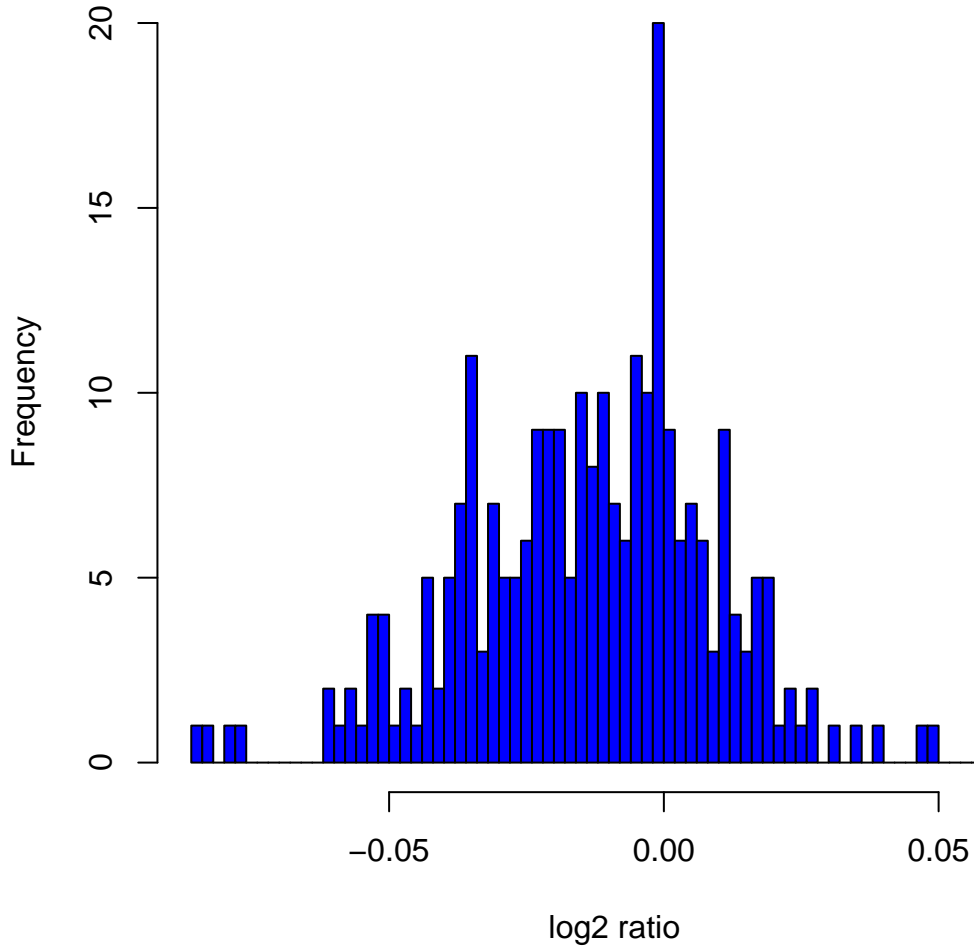
Histogram of log2ratios in 270 HapMap samples at clone Chr12tp-19F3
