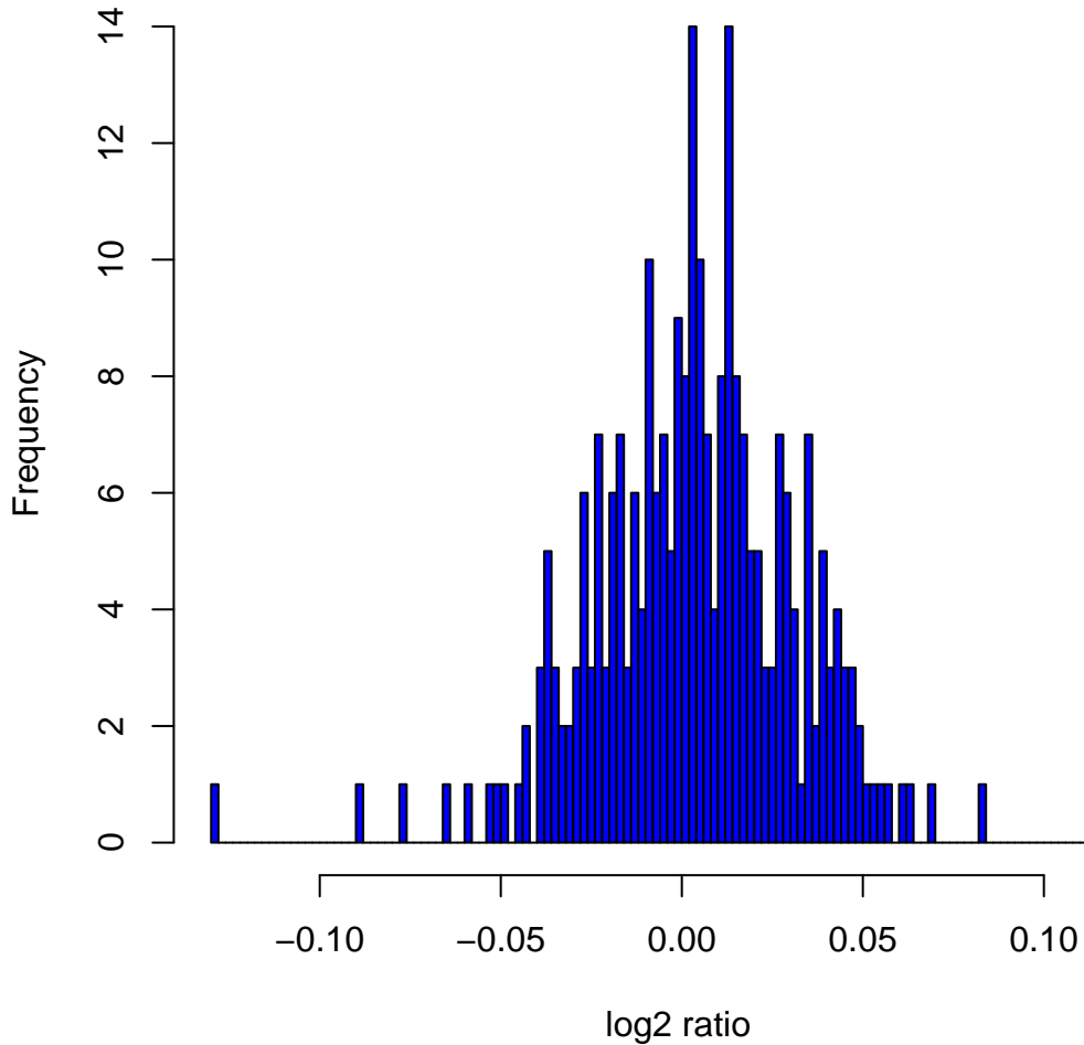
Histogram of log2ratios in 270 HapMap samples at clone Chr12tp-1A8
