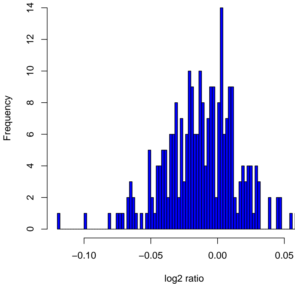
Histogram of log2ratios in 270 HapMap samples at clone Chr12tp-1F4
