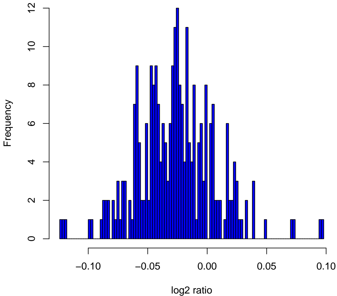
Histogram of log 2 ratios in 270 HapMap samples at clone Chr12tp-1F7
