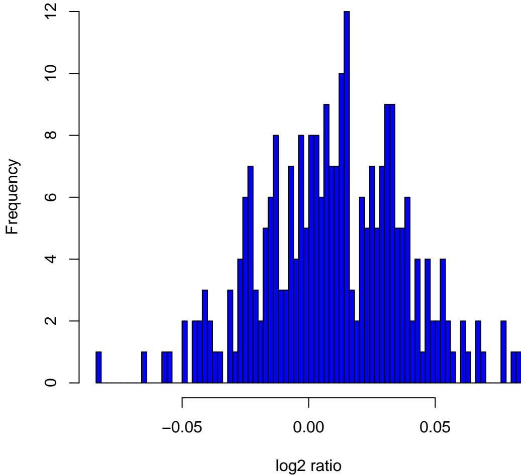
Histogram of log2ratios in 270 HapMap samples at clone Chr12tp-1H11
