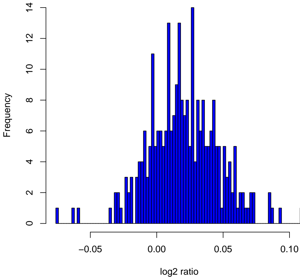
Histogram of log2ratios in 270 HapMap samples at clone Chr12tp-20C9
