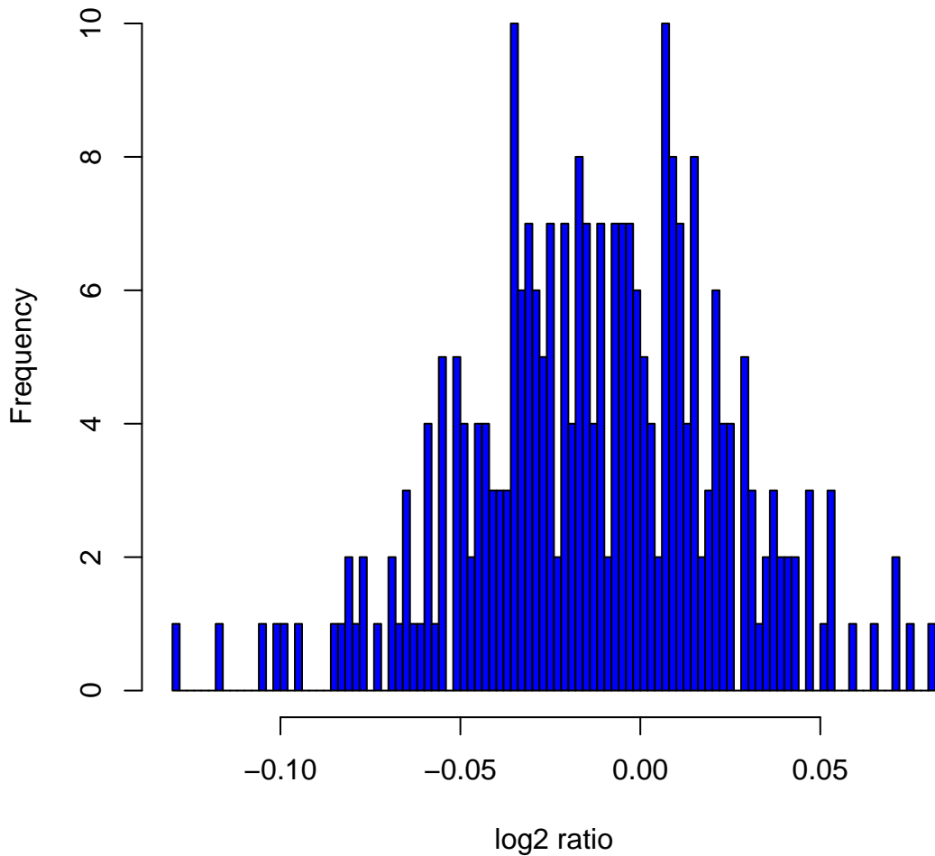
Histogram of \log_2 ratios in 270 HapMap samples at clone Chr12tp-20D5
