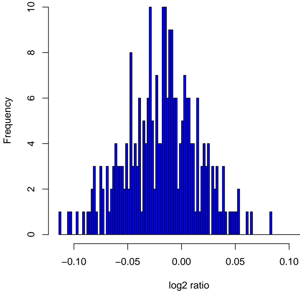
Histogram of log2ratios in 270 HapMap samples at clone Chr12tp-20F9
