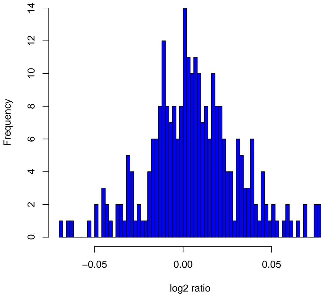
Histogram of log2ratios in 270 HapMap samples at clone Chr12tp-20G11
