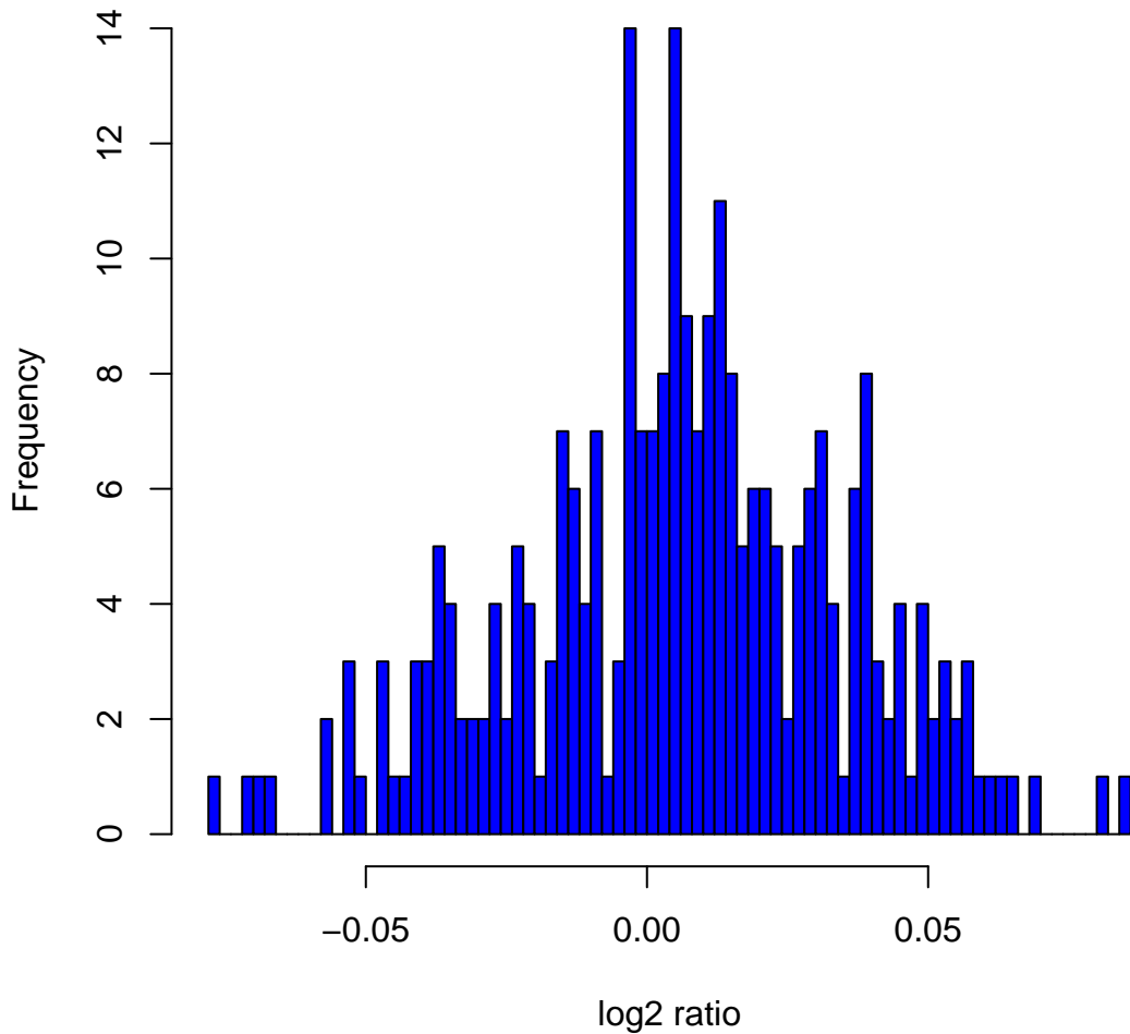
Histogram of log2ratios in 270 HapMap samples at clone Chr12tp-3A12
