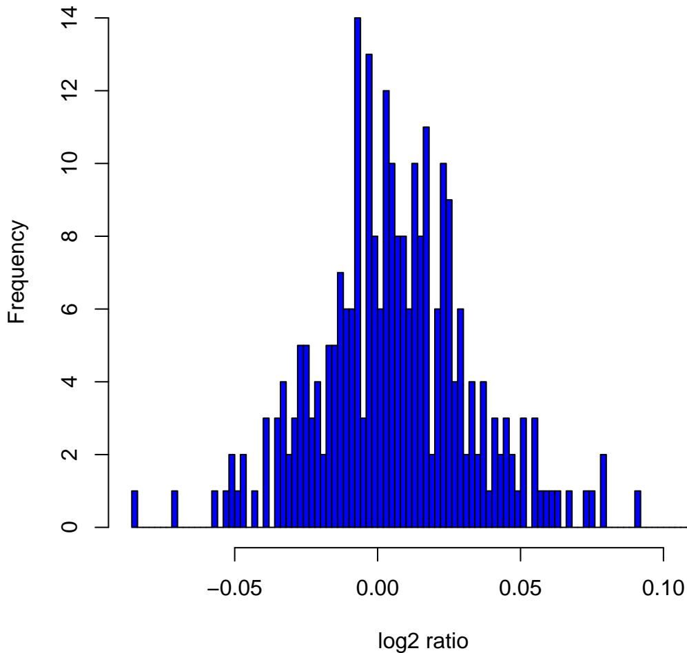
Histogram of log 2 ratios in 270 HapMap samples at clone Chr12tp-3A8
