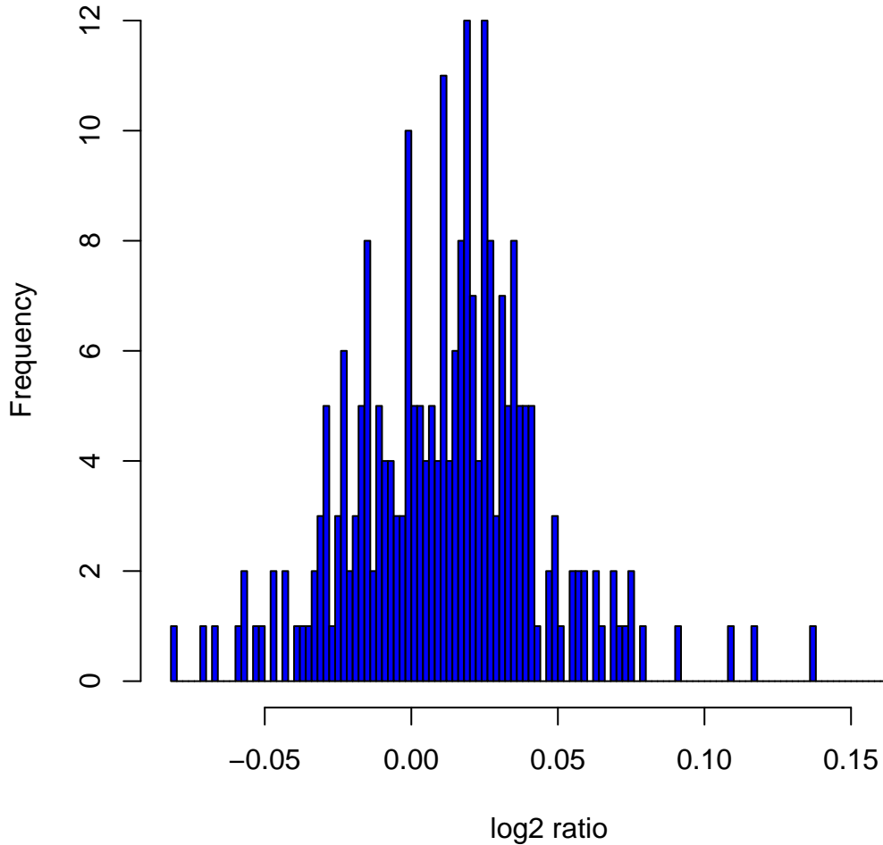
Histogram of log 2 ratios in 270 HapMap samples at clone Chr12tp-3B6
