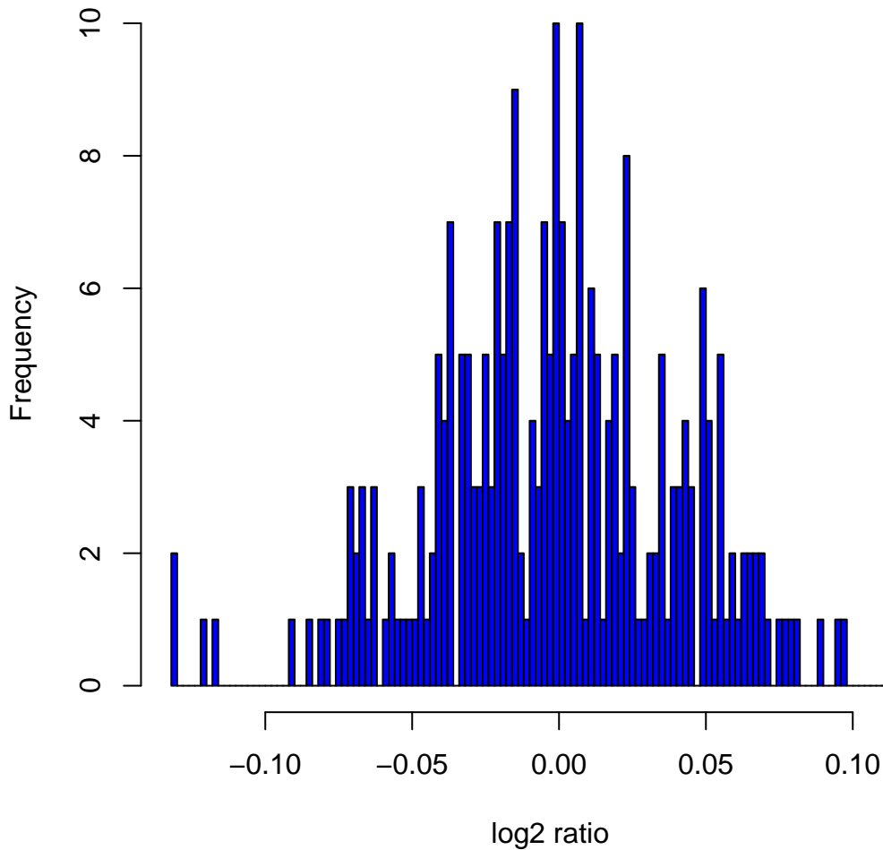
Histogram of log 2 ratios in 270 HapMap samples at clone Chr12tp-3D2
