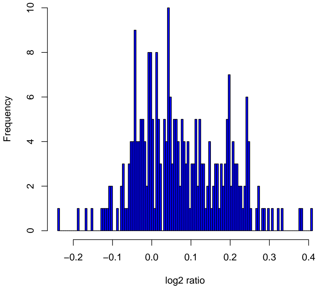
Histogram of \log_2 ratios in 270 HapMap samples at clone Chr12tp-3E1
