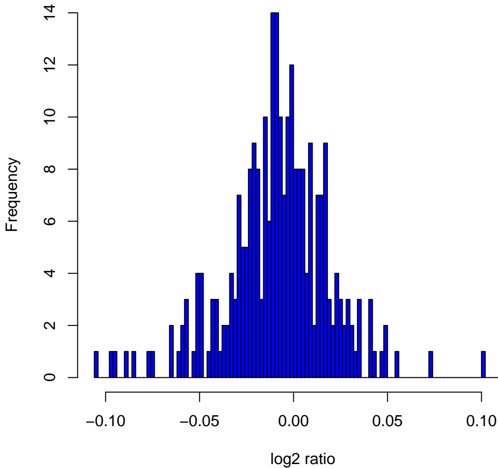
Histogram of log 2 ratios in 270 HapMap samples at clone Chr12tp-3E6
