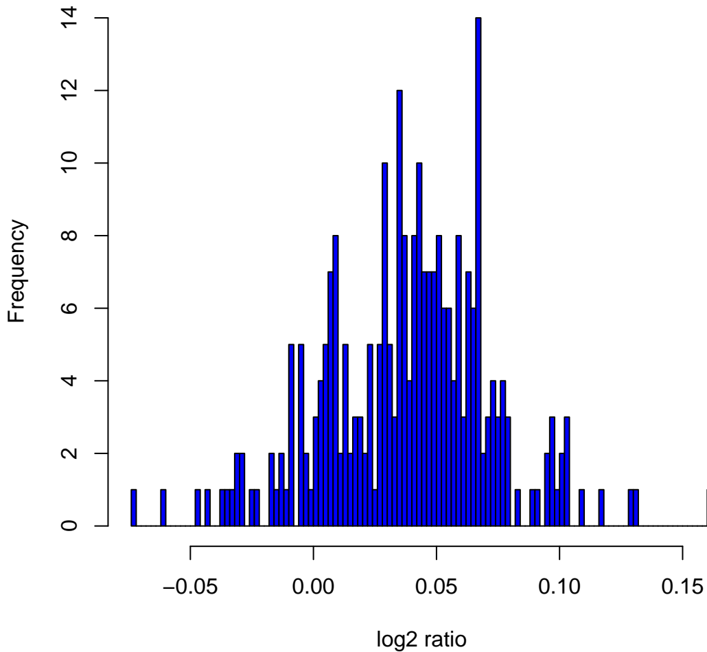
Histogram of log 2 ratios in 270 HapMap samples at clone Chr12tp-3G7
