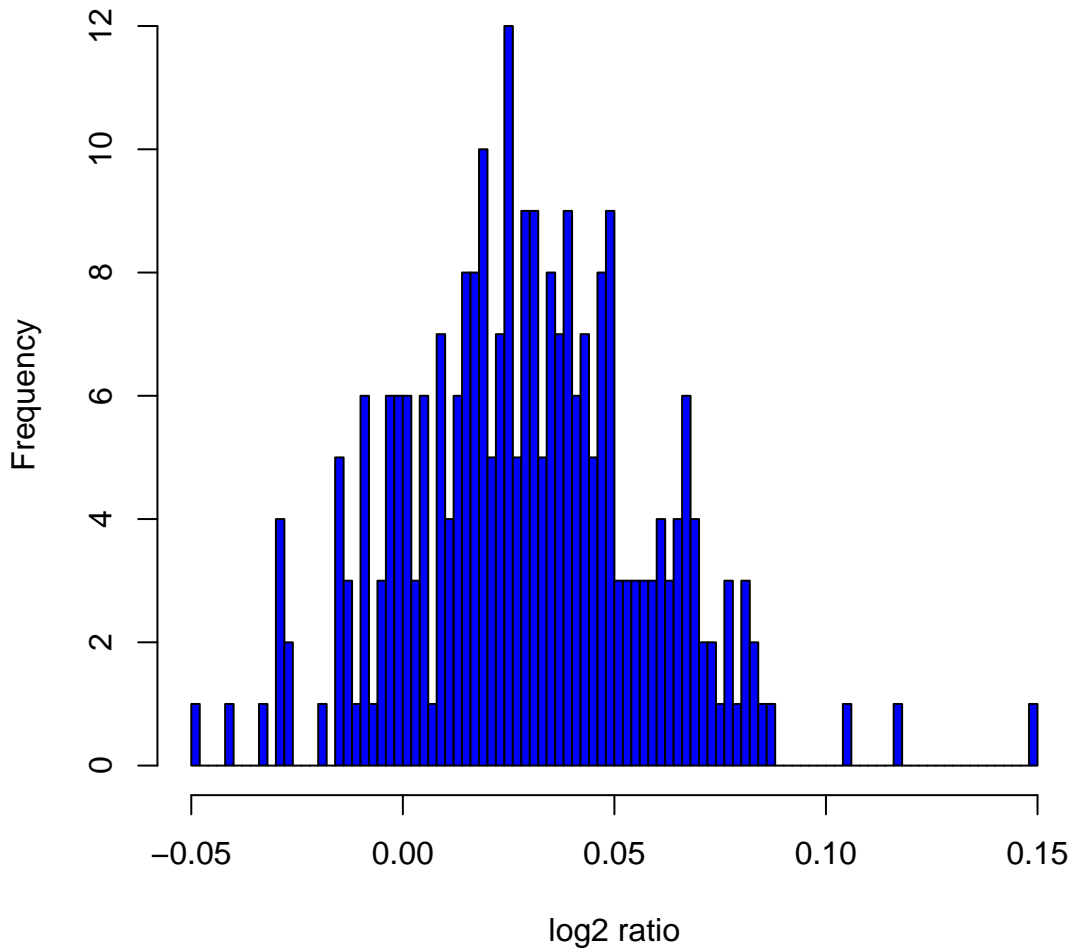
Histogram of \log_2 ratios in 270 HapMap samples at clone Chr12tp-3G8
