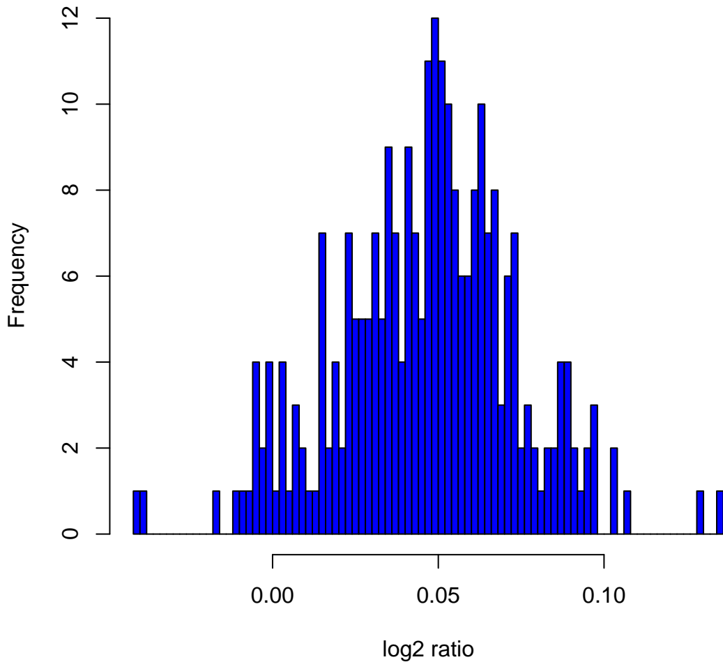
Histogram of log2ratios in 270 HapMap samples at clone Chr12tp-4A11
