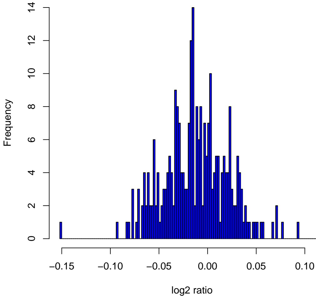
Histogram of log2ratios in 270 HapMap samples at clone Chr12tp-4A4
