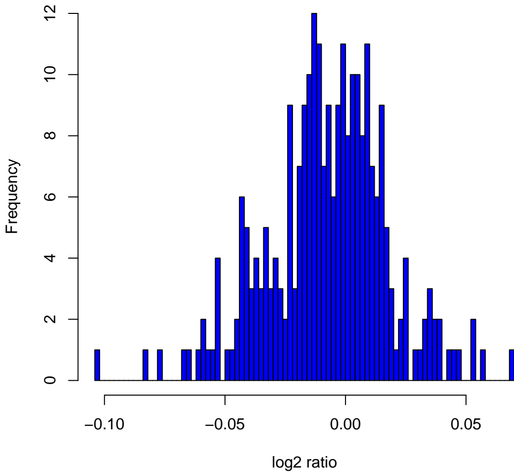
Histogram of log 2 ratios in 270 HapMap samples at clone Chr12tp-4B6
