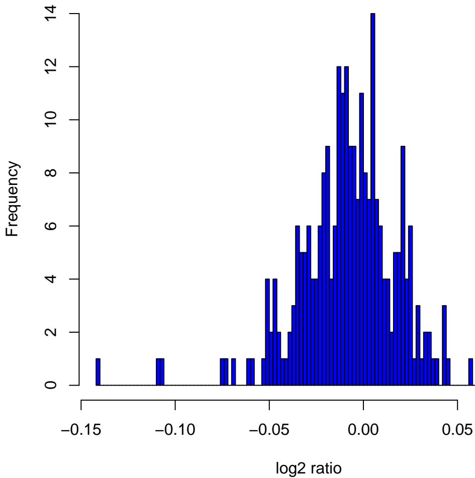
Histogram of log 2 ratios in 270 HapMap samples at clone Chr12tp-4D6
