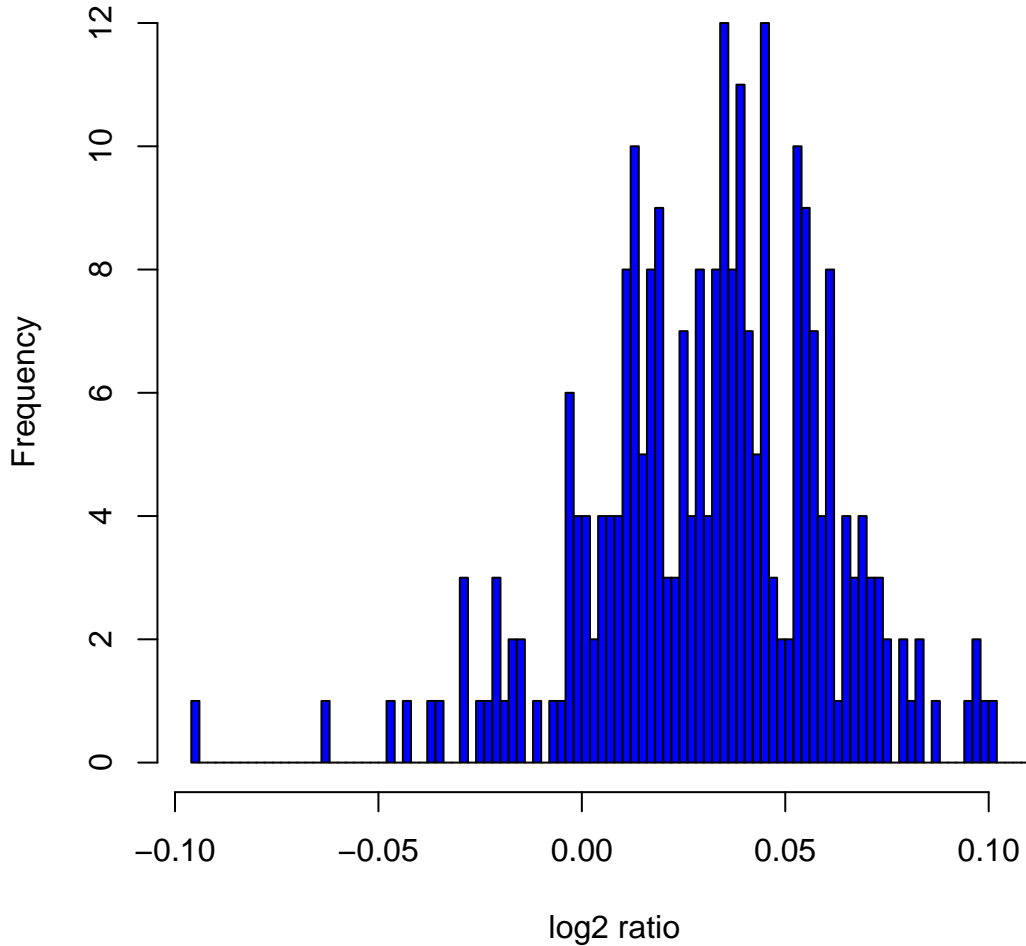
Histogram of log 2 ratios in 270 HapMap samples at clone Chr12tp-4G5
