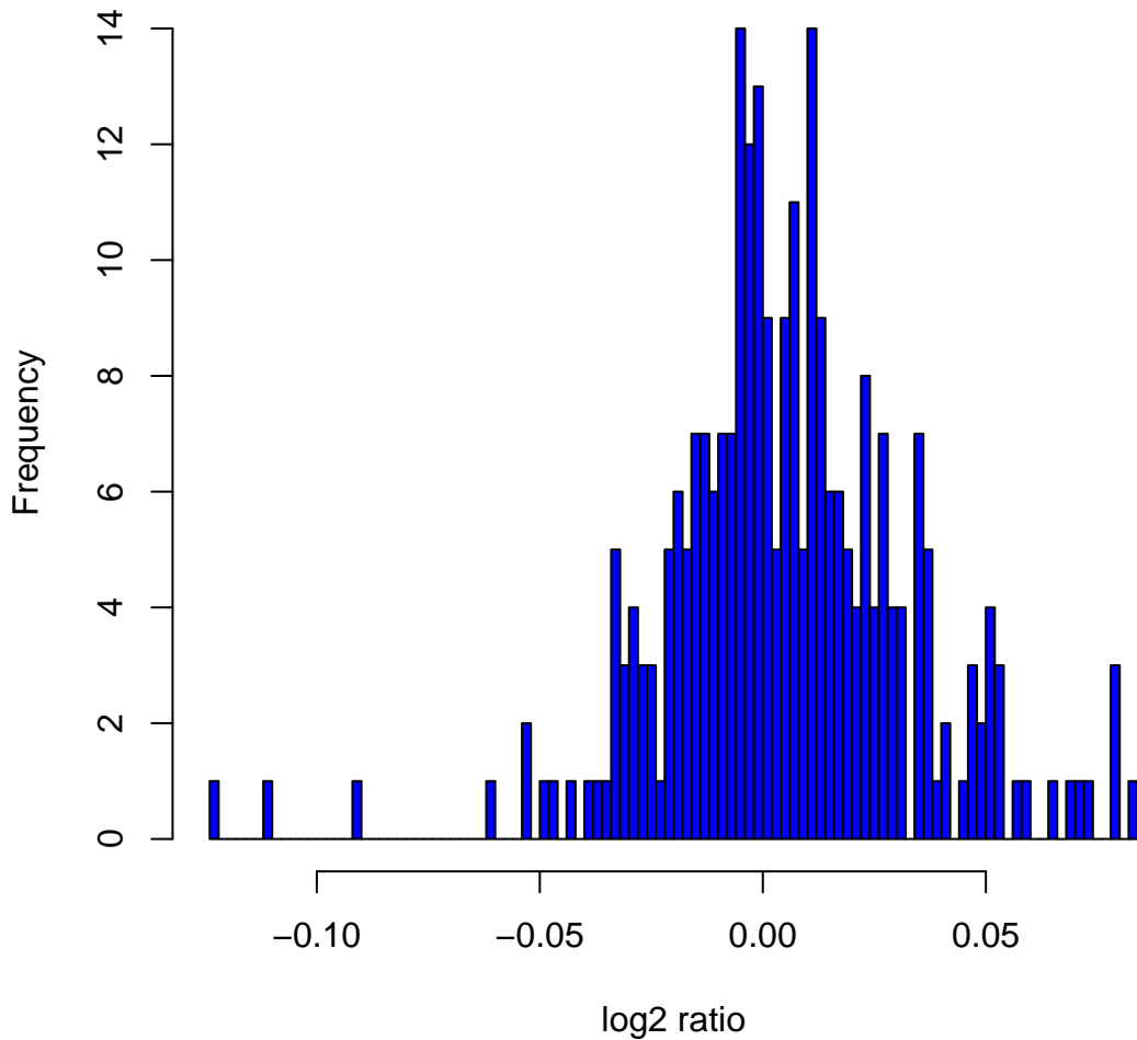
Histogram of log 2 ratios in 270 HapMap samples at clone Chr12tp-4G9
