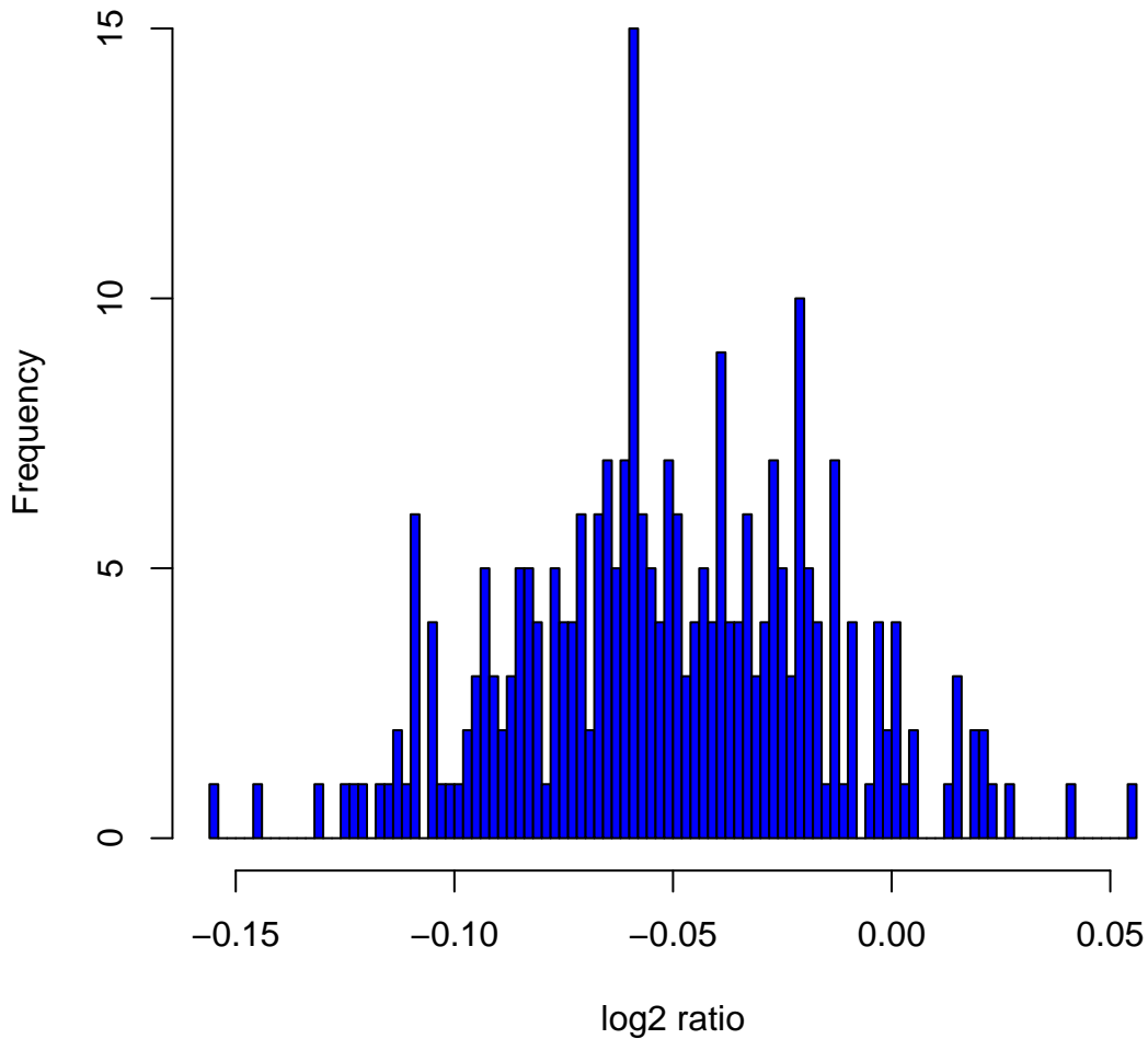
Histogram of log2ratios in 270 HapMap samples at clone Chr12tp-5D10
