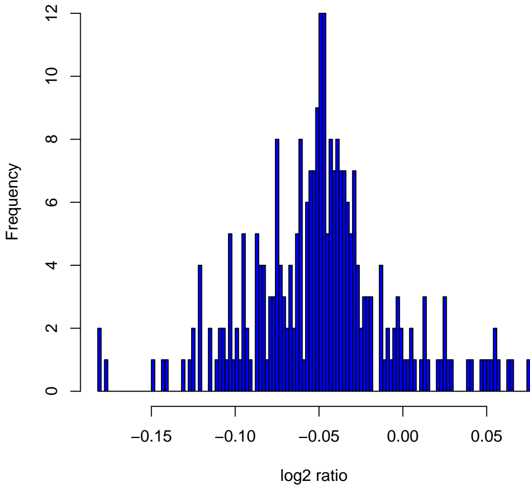
Histogram of log 2 ratios in 270 HapMap samples at clone Chr12tp-5G3
