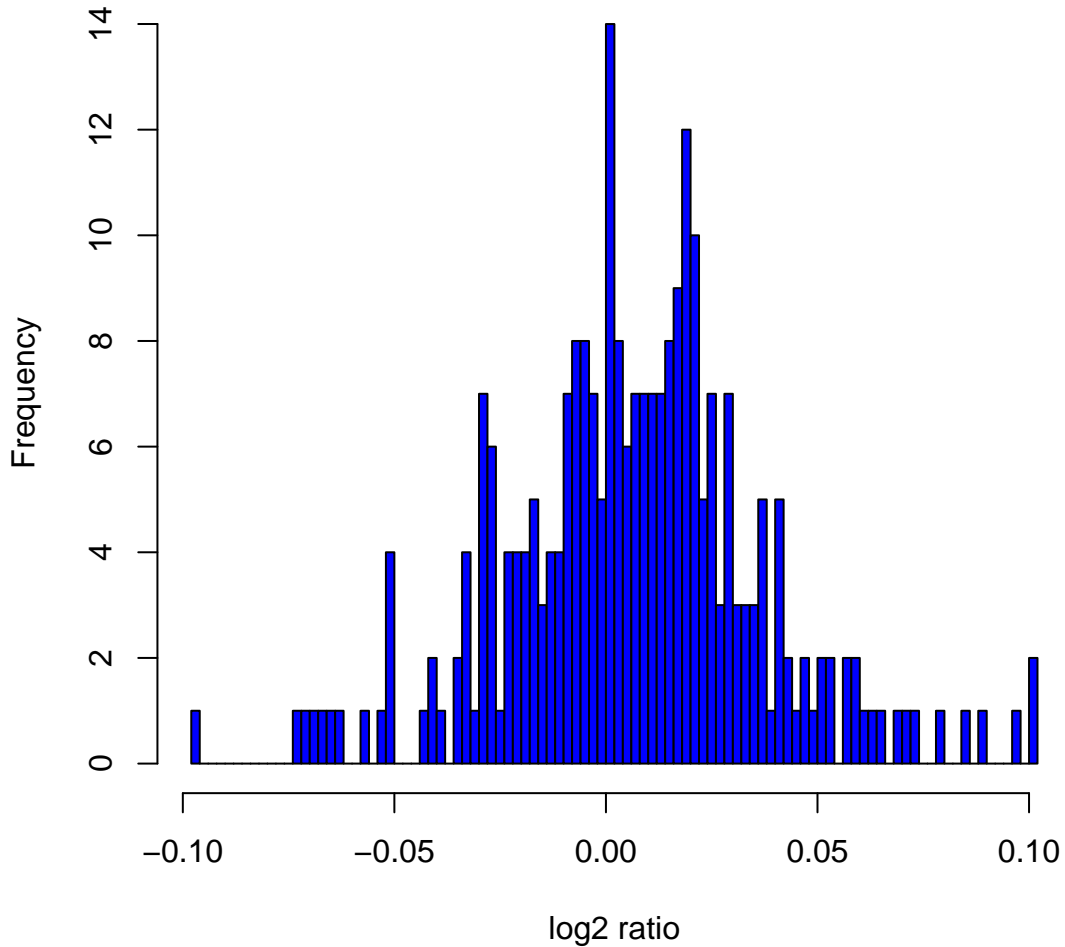
Histogram of log 2 ratios in 270 HapMap samples at clone Chr12tp-6D2
