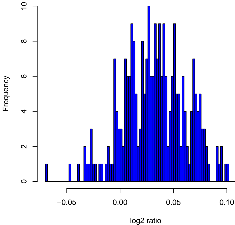
Histogram of log 2 ratios in 270 HapMap samples at clone Chr12tp-6D9
