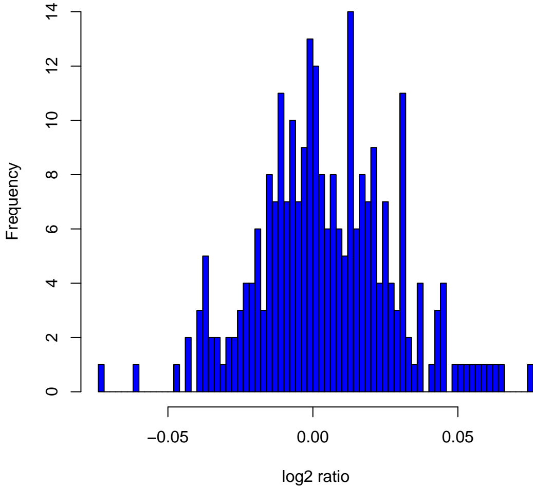
Histogram of log2ratios in 270 HapMap samples at clone Chr12tp-6G11
