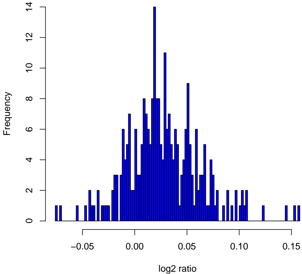
Histogram of log2ratios in 270 HapMap samples at clone Chr12tp-6H2
