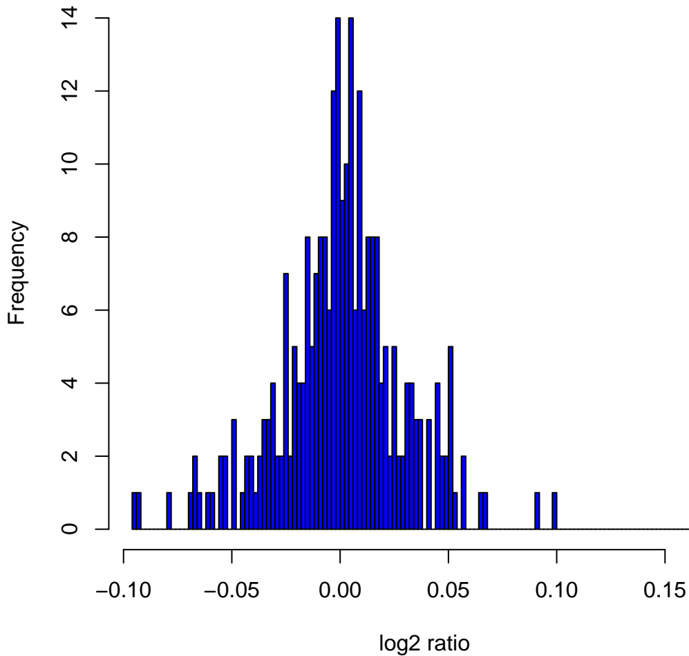
Histogram of log 2 ratios in 270 HapMap samples at clone Chr12tp-6H5
