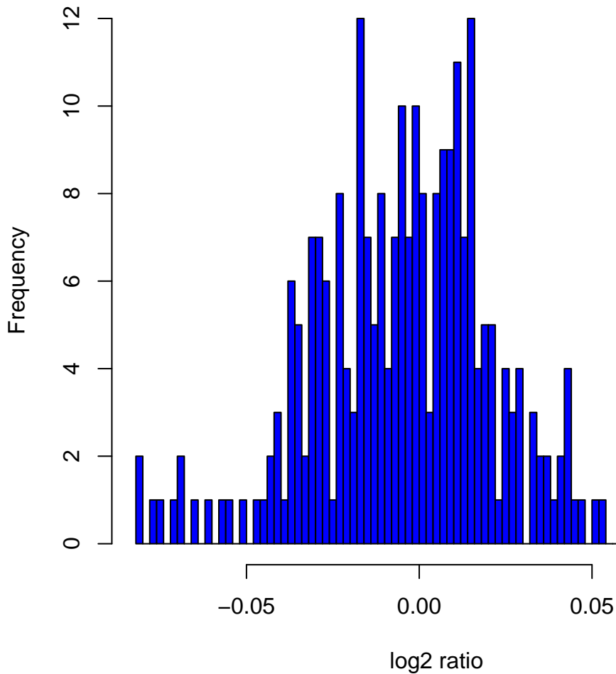
Histogram of log 2 ratios in 270 HapMap samples at clone Chr12tp-6H7
