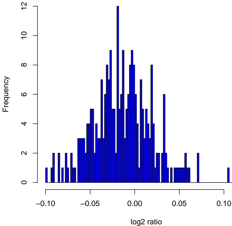
Histogram of log 2 ratios in 270 HapMap samples at clone Chr12tp-7B3
