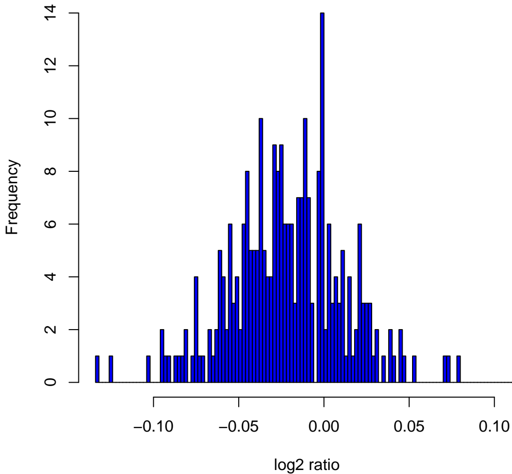
Histogram of log 2 ratios in 270 HapMap samples at clone Chr12tp-7B6
